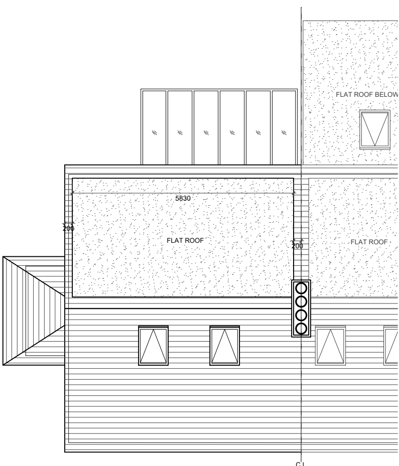
03 - ROOF PLAN
