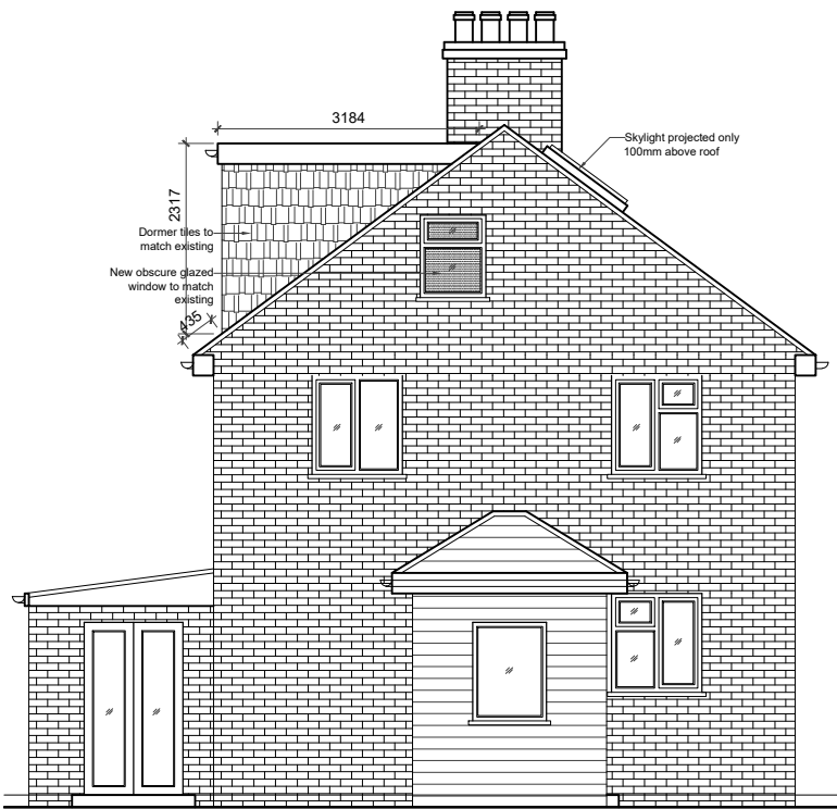
06 - SIDE ELEVATION
