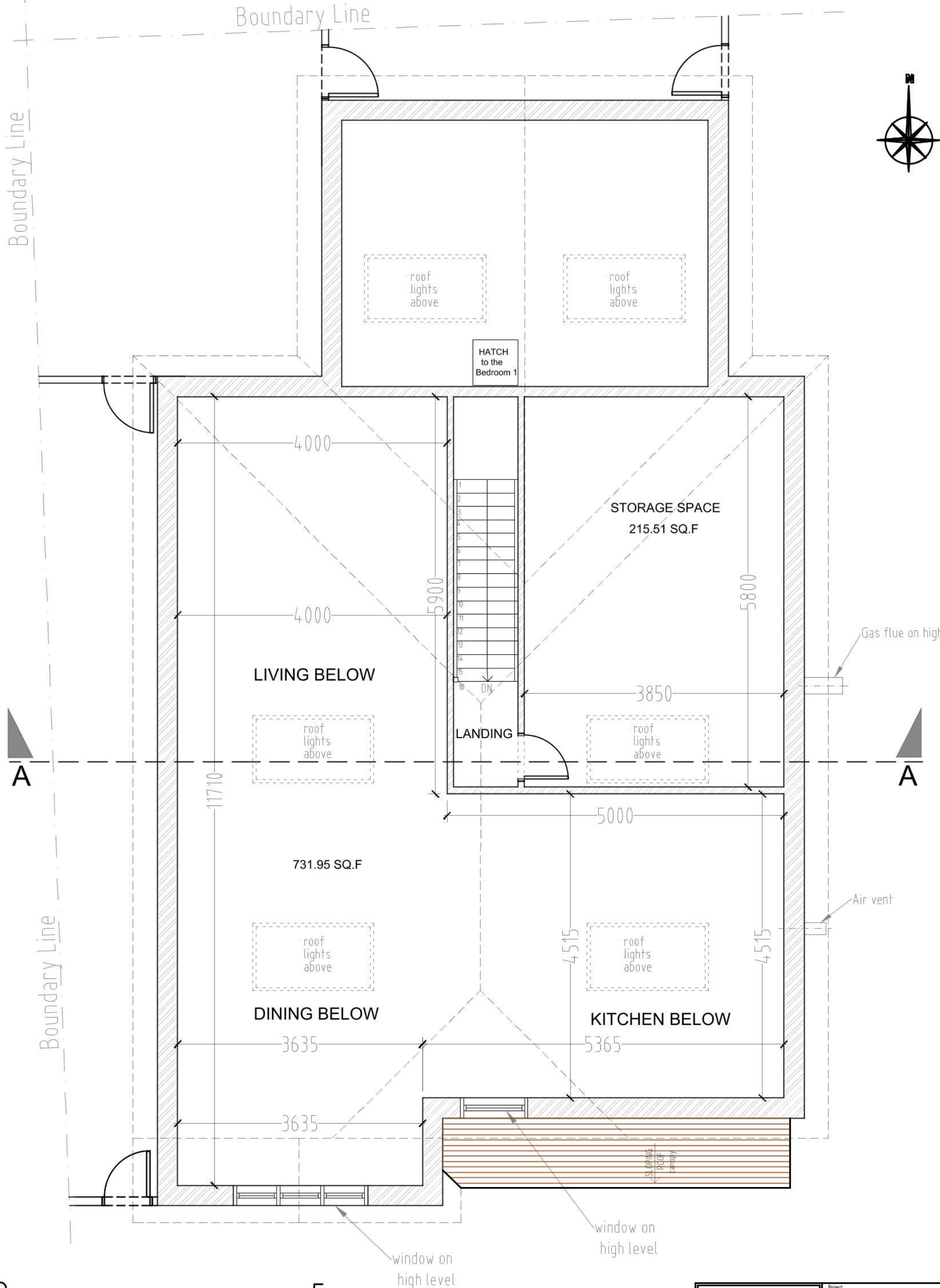
PROPOSED ATTIC PLAN @ SCALE 1:50 @ A3
