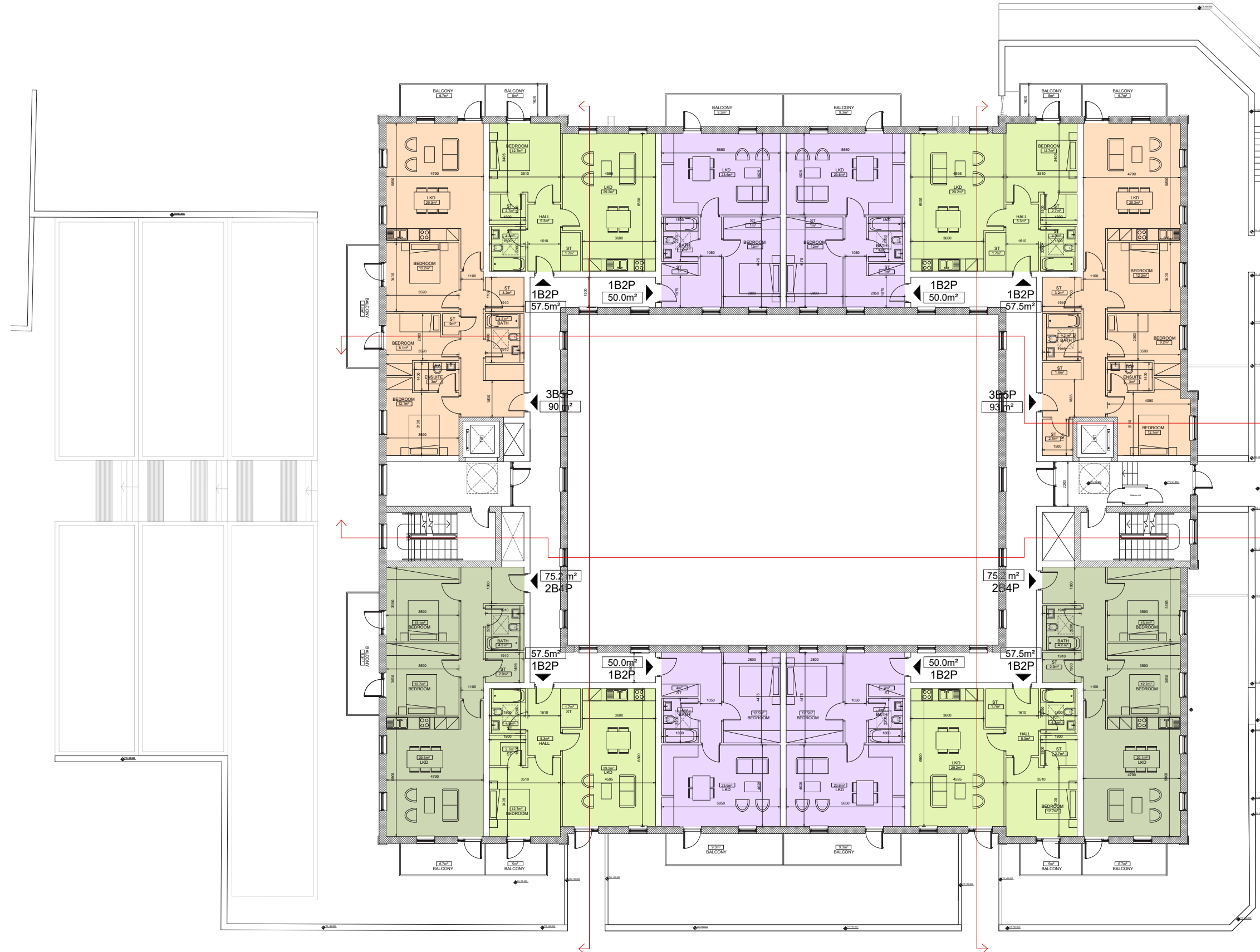
FIG 15 Stable House Ground Floor Plan
