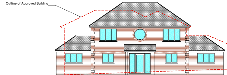
NORTHWEST ELEVATION
