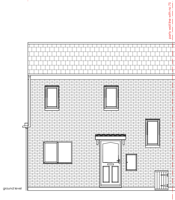
NORTH - EAST ELEVATION
