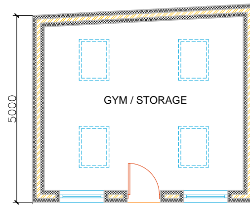
PROPOSED OUT-BUILDING
