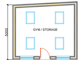
PROPOSED OUT-BUILDING
