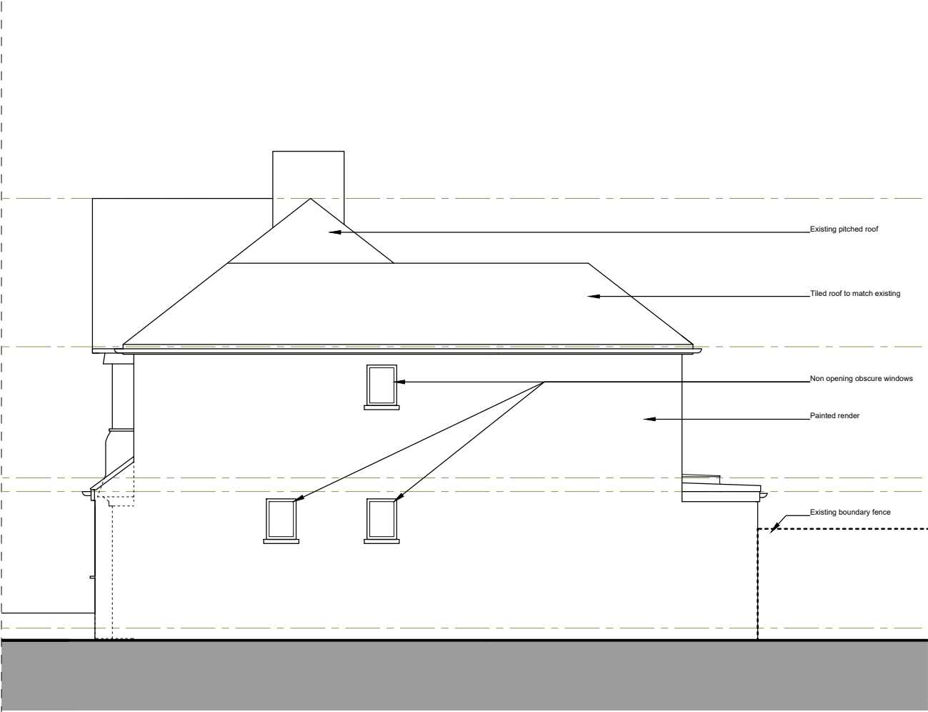
SIDE ELEVATION
