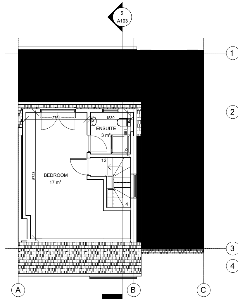
PROPOSED LOFT PLAN
