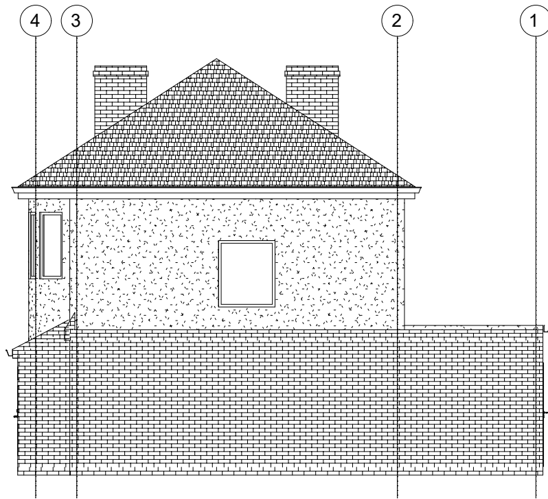
EXISTING RIGHT SIDE ELEVATION
