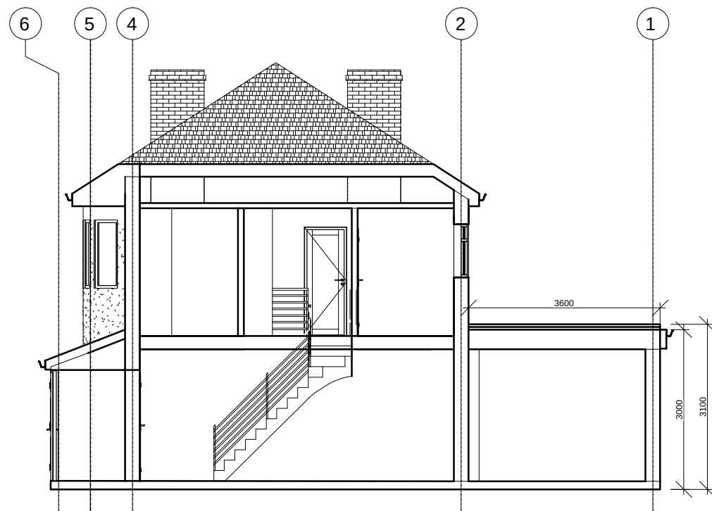
PROPOSED SECTION
