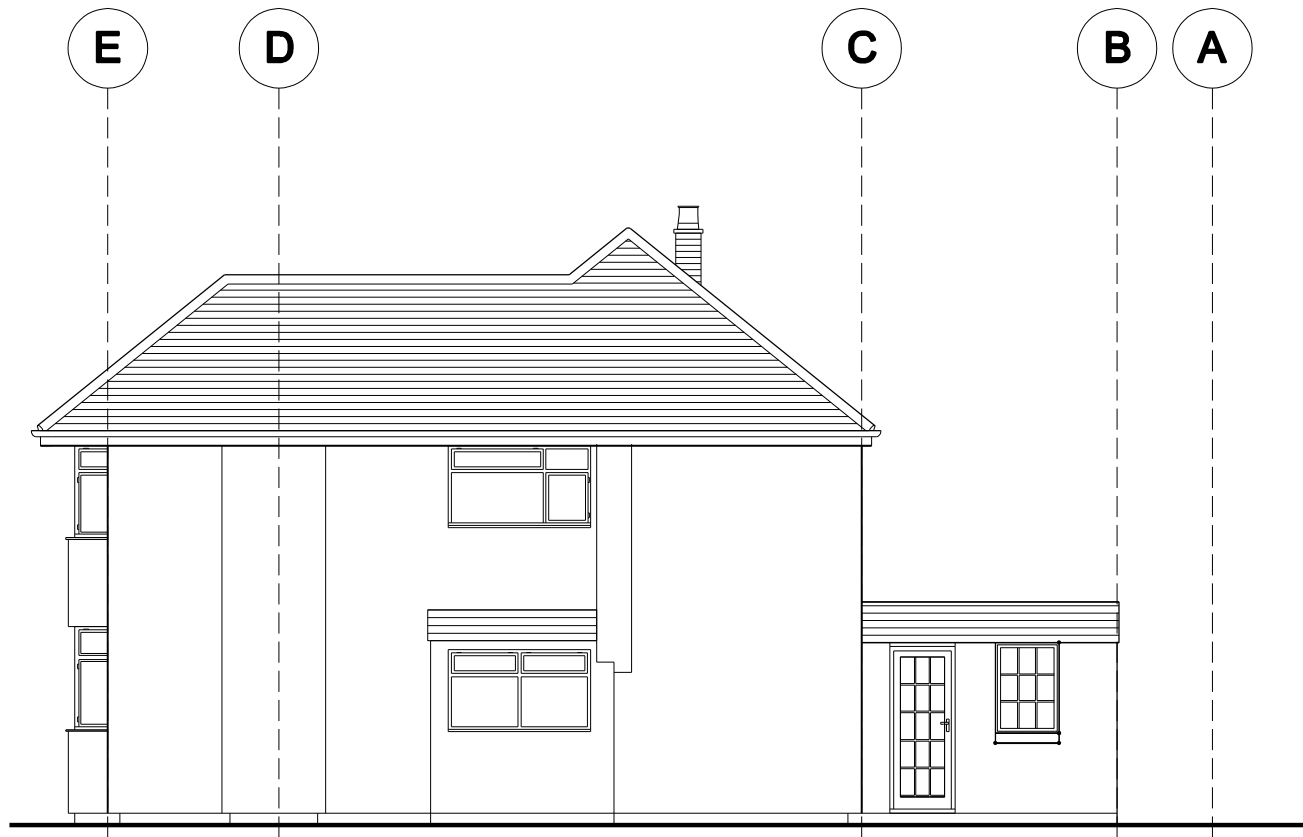
01 EXISTING SIDE ELEVATION SCALE 1:100
