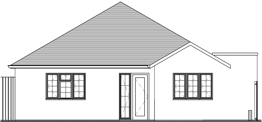
Proposed Front Elevation 1 : 100
