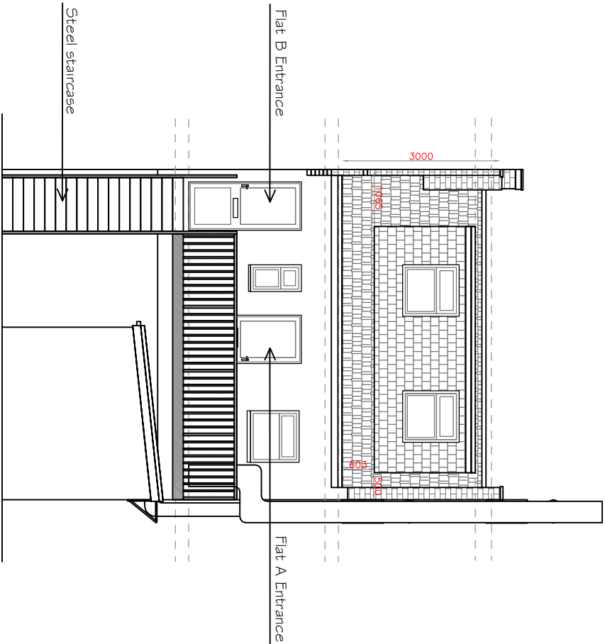
PROPOSED REAR ELEVATION 1:100 A3
