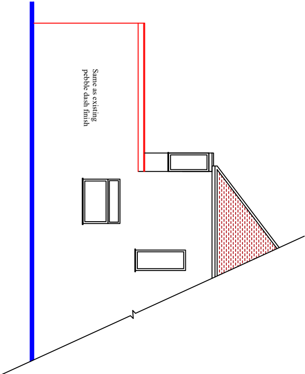
LEFT SIDE ELEVATION (Proposed)
