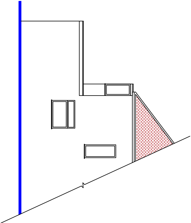
LEFT SIDE ELEVATION (Existing)
