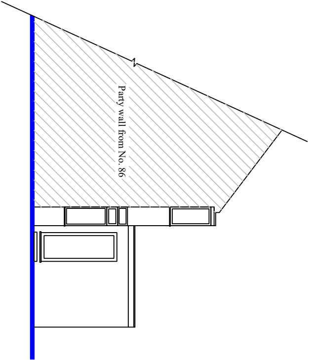
RIGHT SIDE ELEVATION (Existing)
