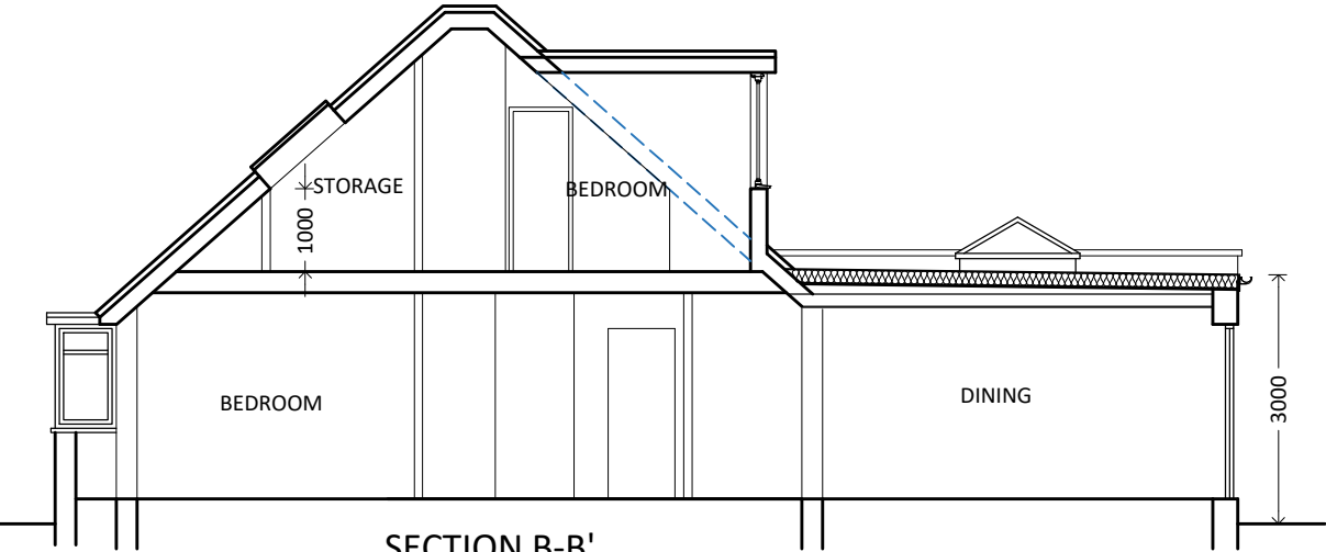
SECTION B-B'
