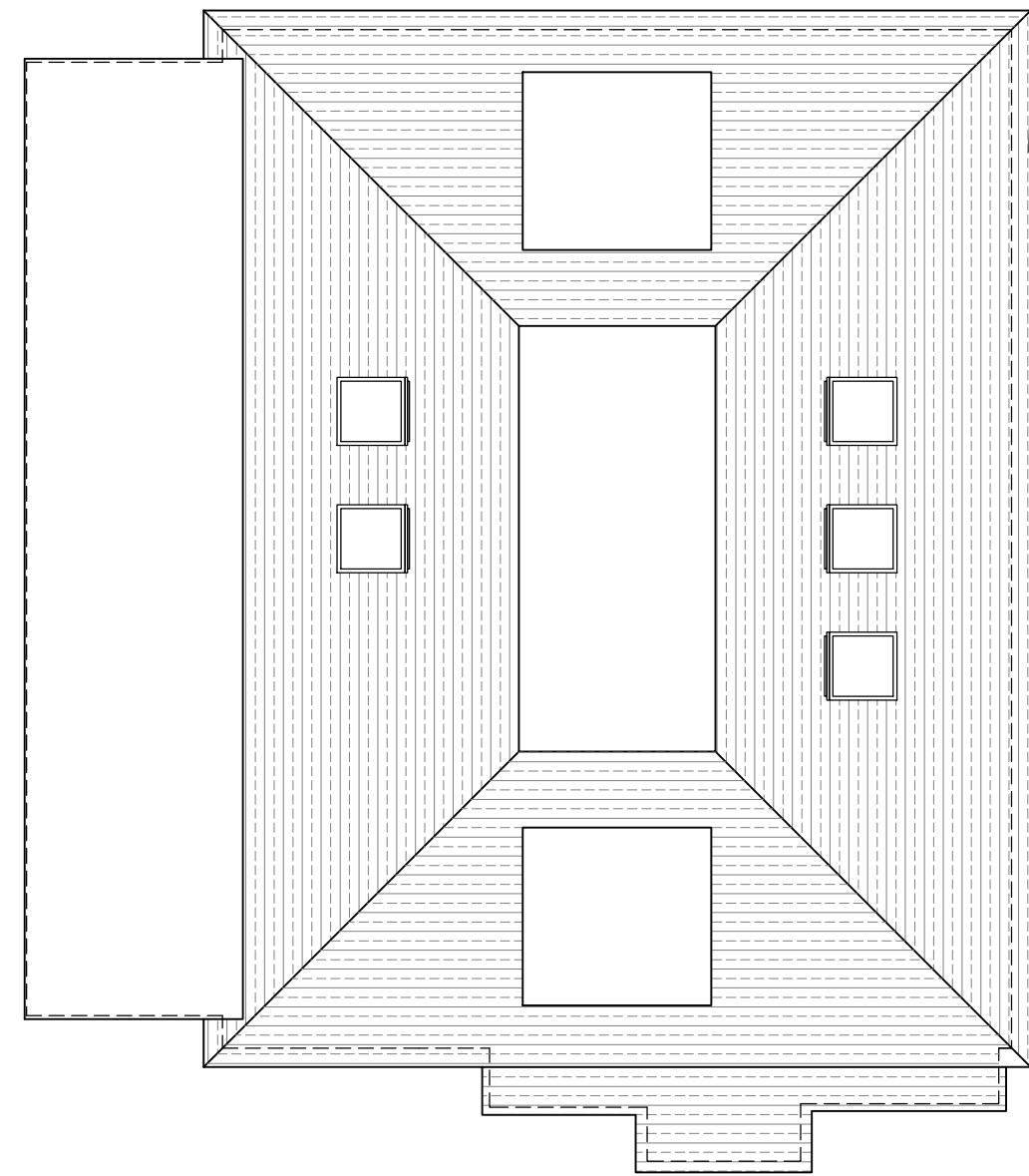
ROOF PLAN
