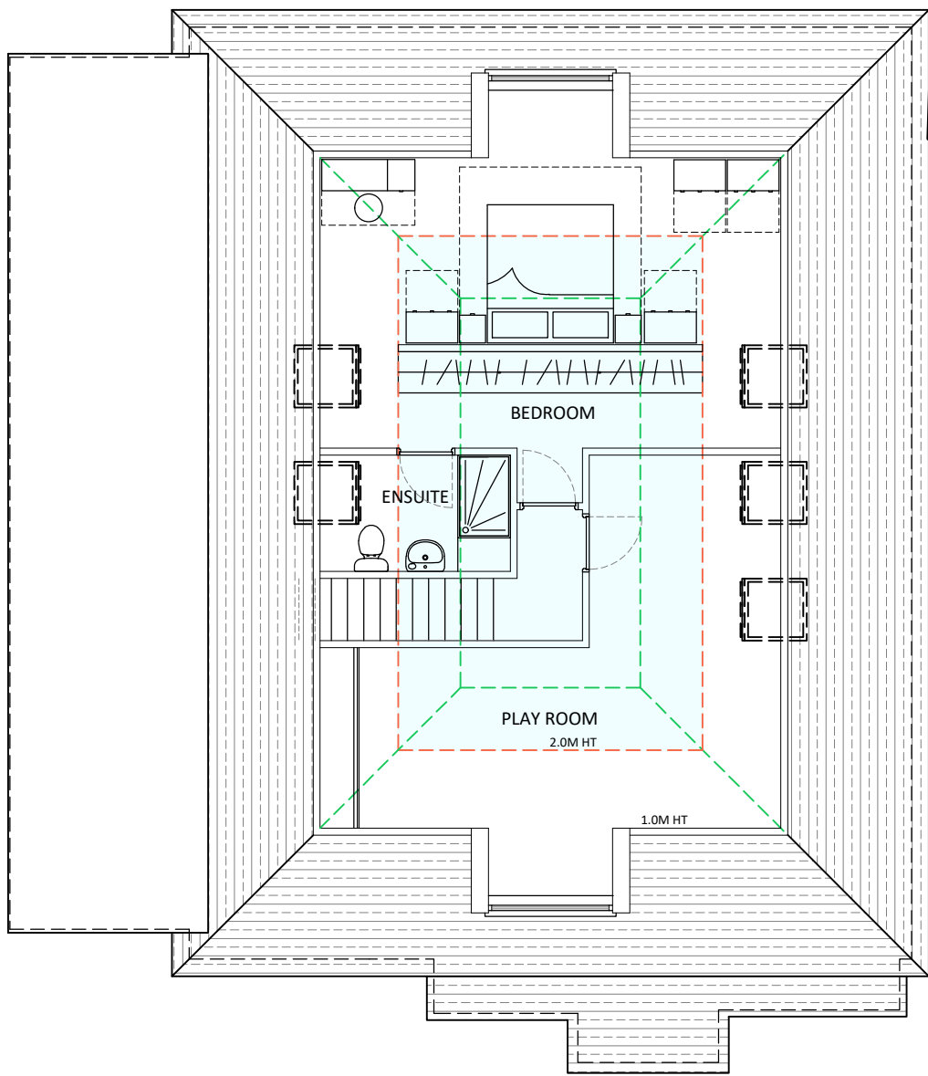
LOFT PLAN --- DENOTES 2.0M HEIGHT
