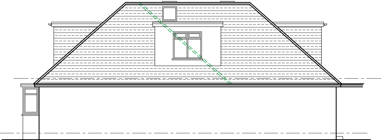
SIDE ELEVATION FACING No 89
