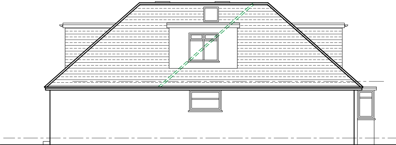
SIDE ELEVATION FACING No 85
