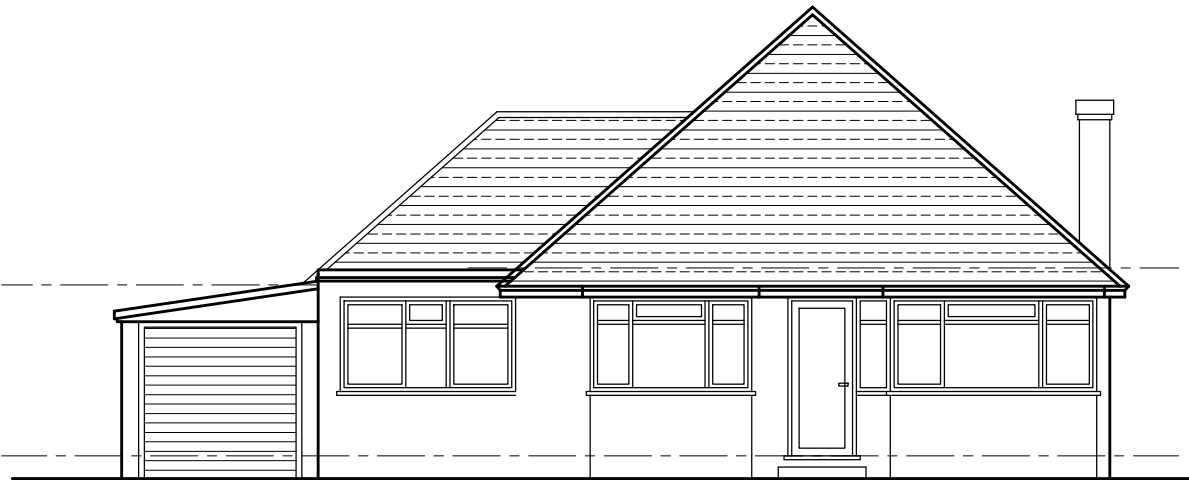
FRONT ELEVATION
