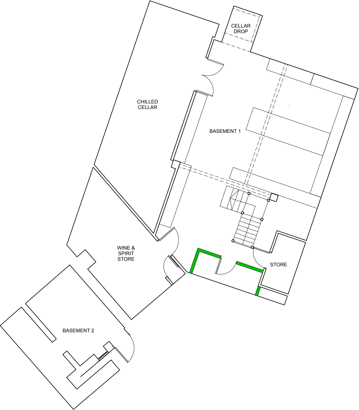
01 PROPOSED BASEMENT PLAN 1:50 @ A1 / 1:100 @ A3
