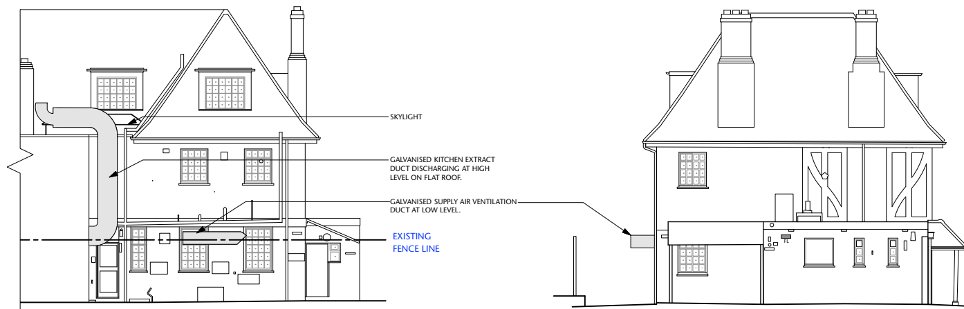
05 EXISTING ELEVATION 5 1:100 @ A1
