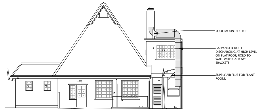
04 EXISTING ELEVATION 4 1:100 @ A1
