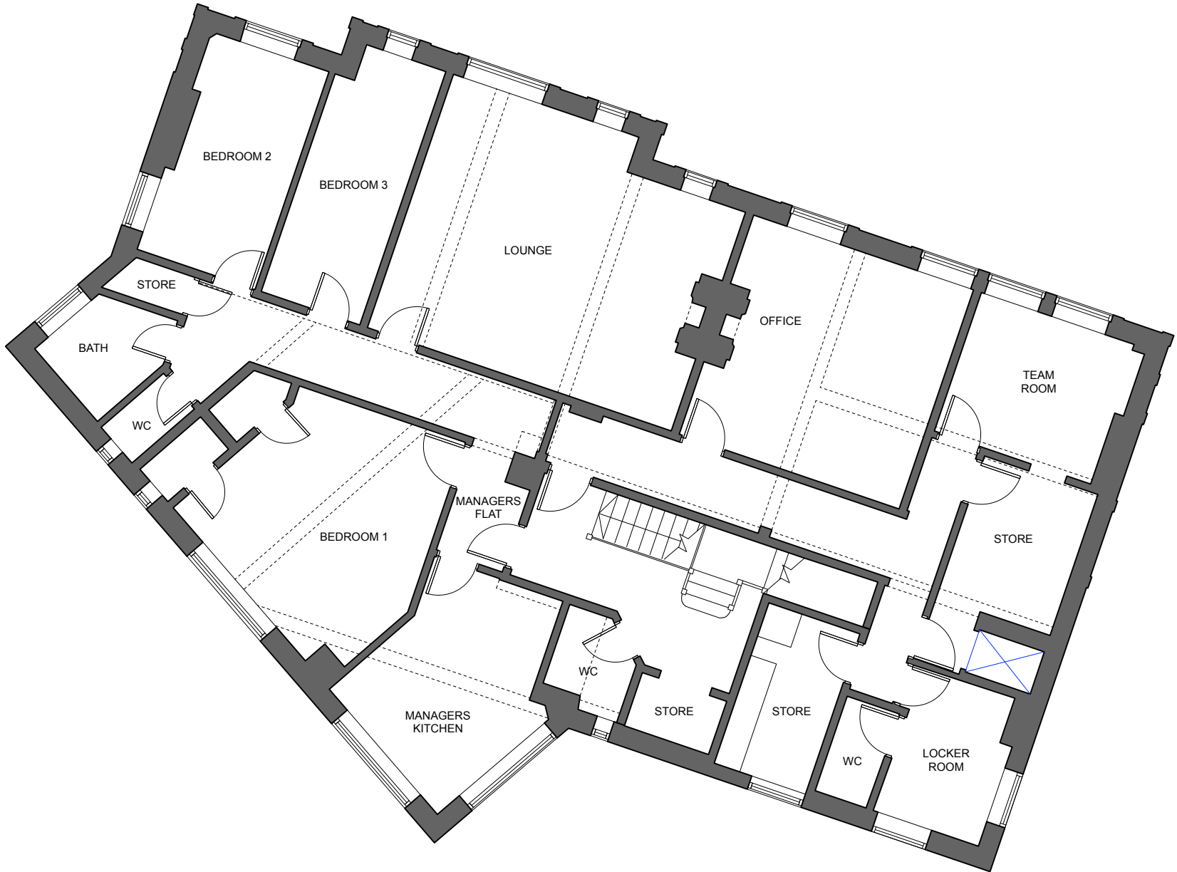
01 EXISTING FIRST FLOOR PLAN 1:50 @ A1 / 1:100 @ A3
