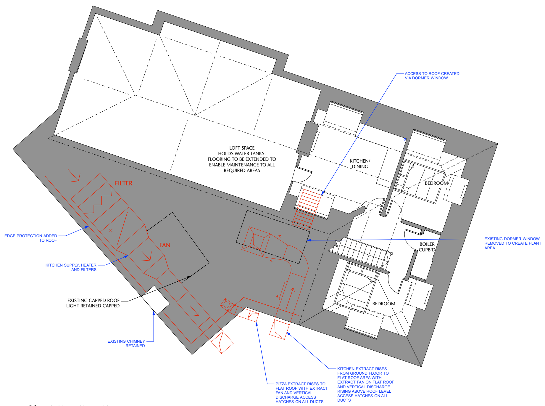
01 PROPOSED SECOND FLOOR PLAN 1:50 @ A1 / 1:100 @ A3
