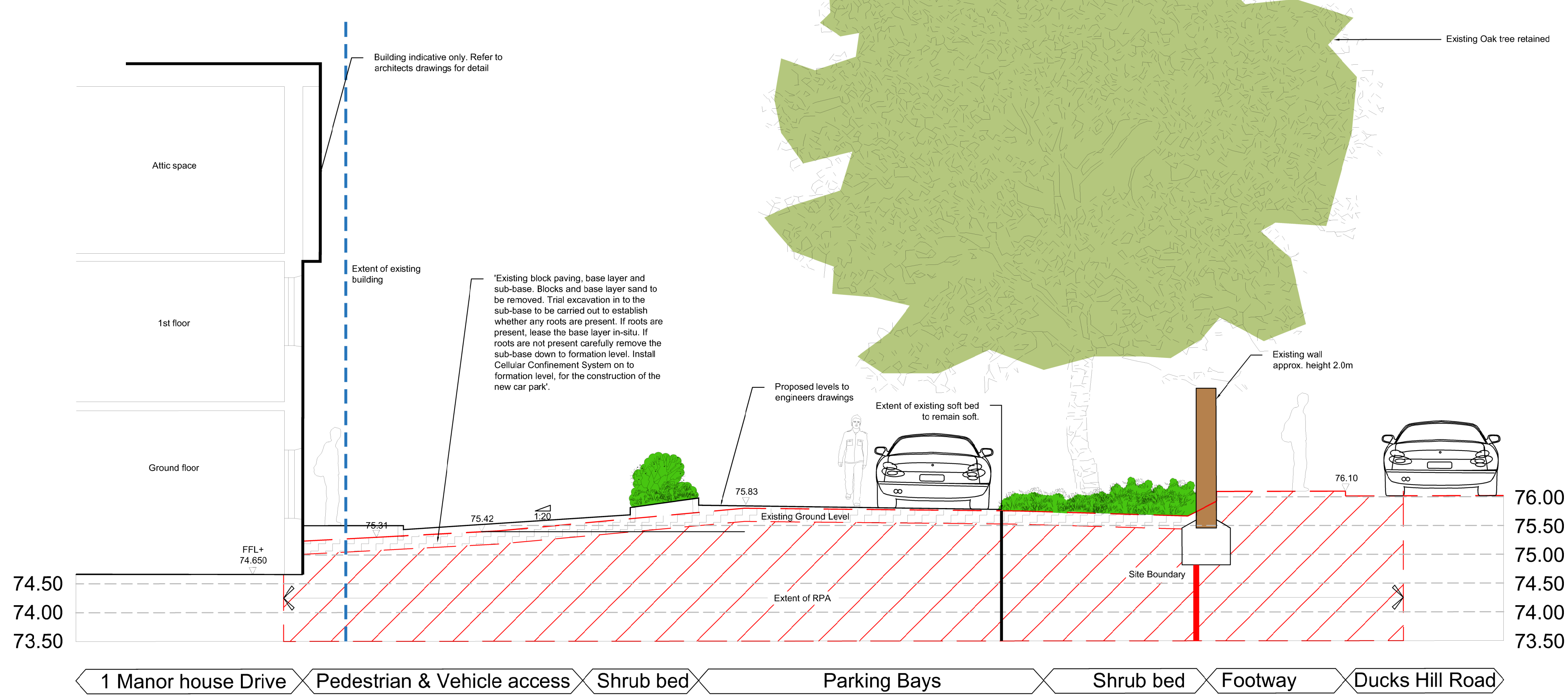
SECTION A-A - Entrance to boundary through car park & TPO oak tree Scale 1:50
