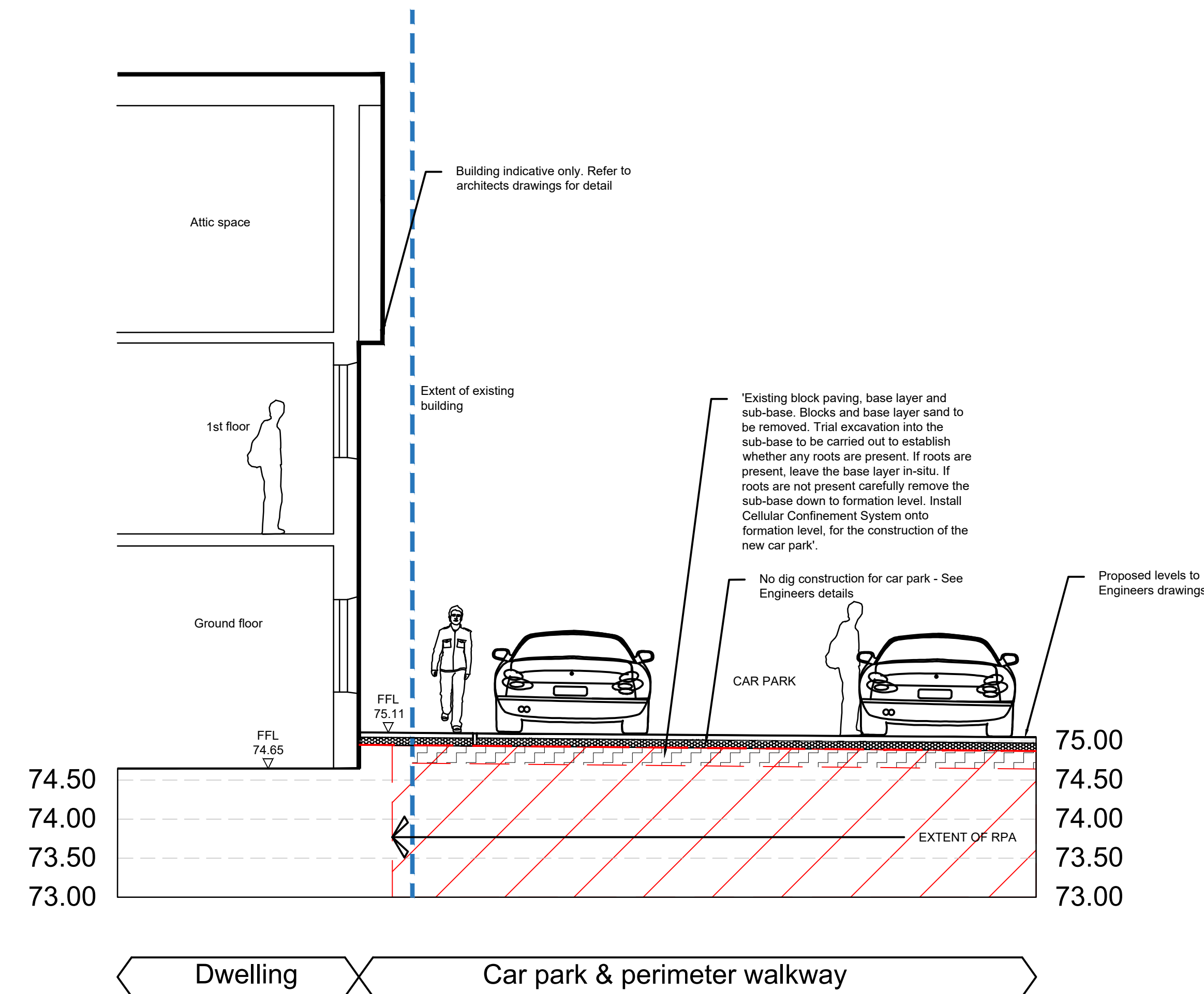
SECTION C-C - Section through bay window & car park Scale 1:50
