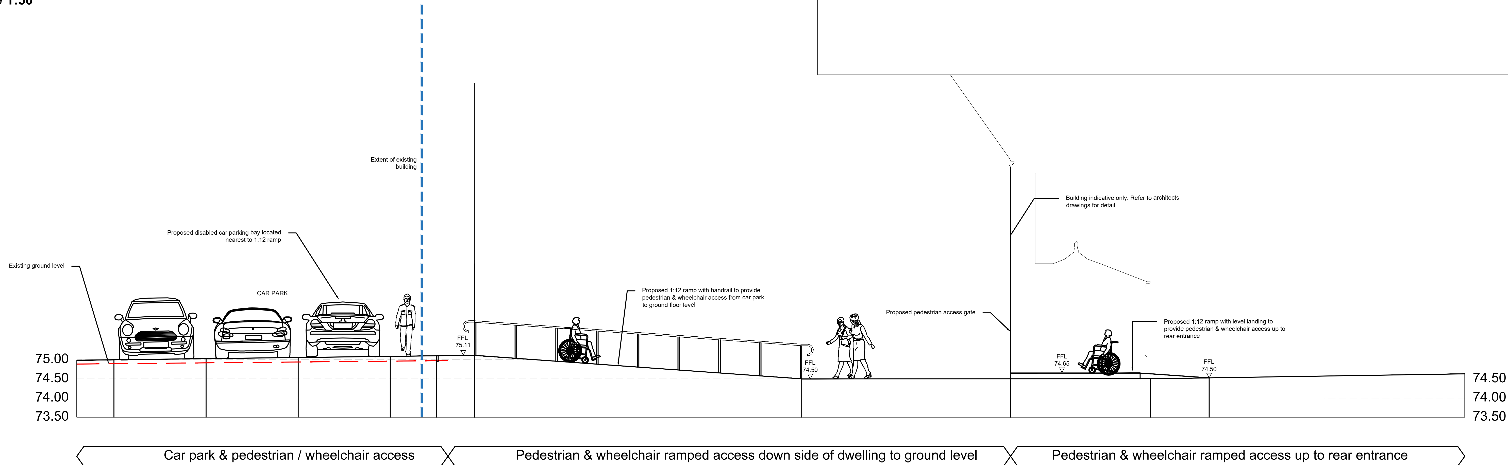
ELEVATION E-E - car park & ramped access down side of dwelling Scale 1:50
