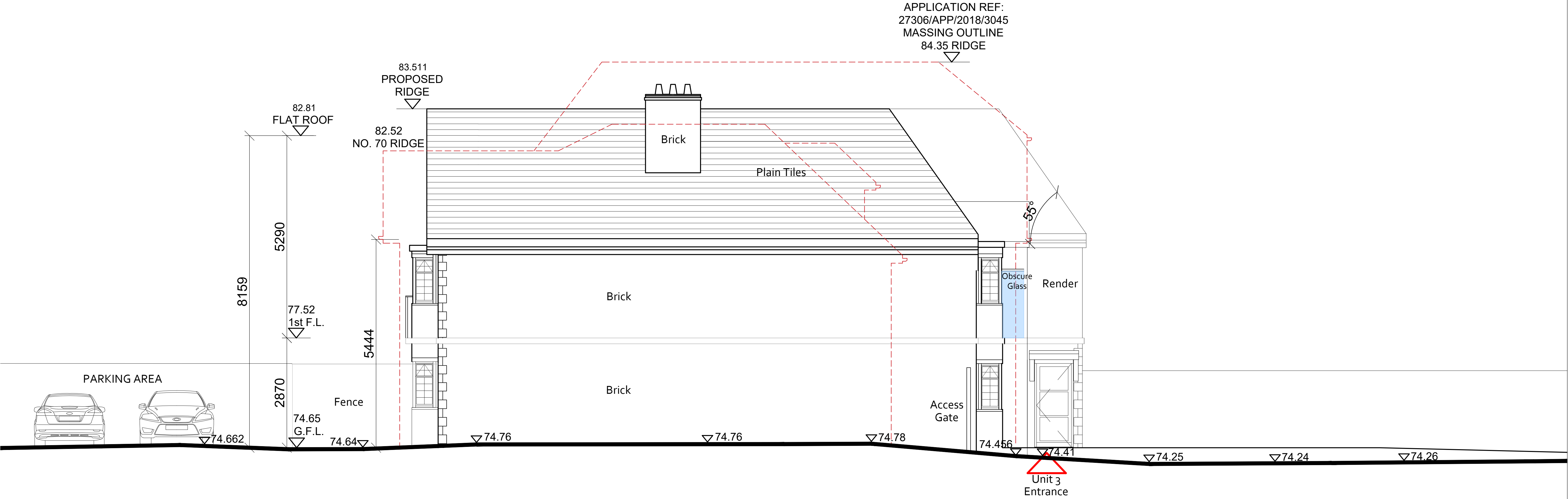
1 Proposed North-East Facing Elevation
