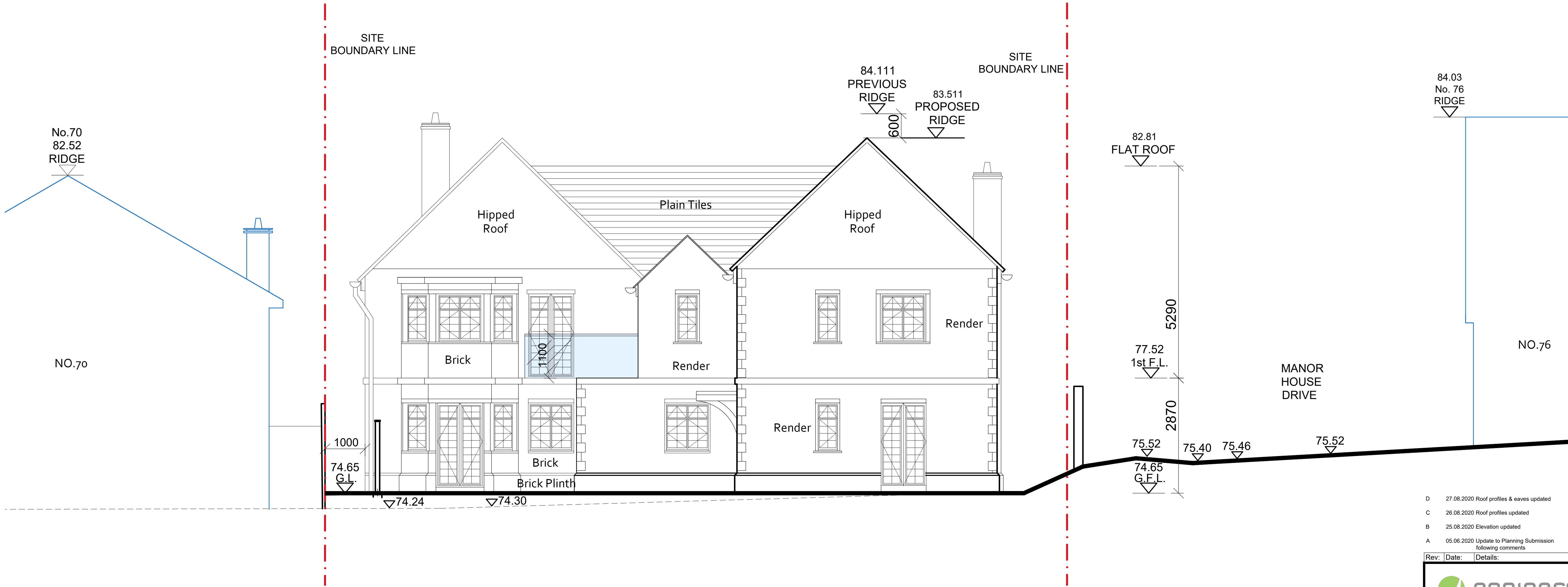
1 Proposed North-West Facing Elevation
