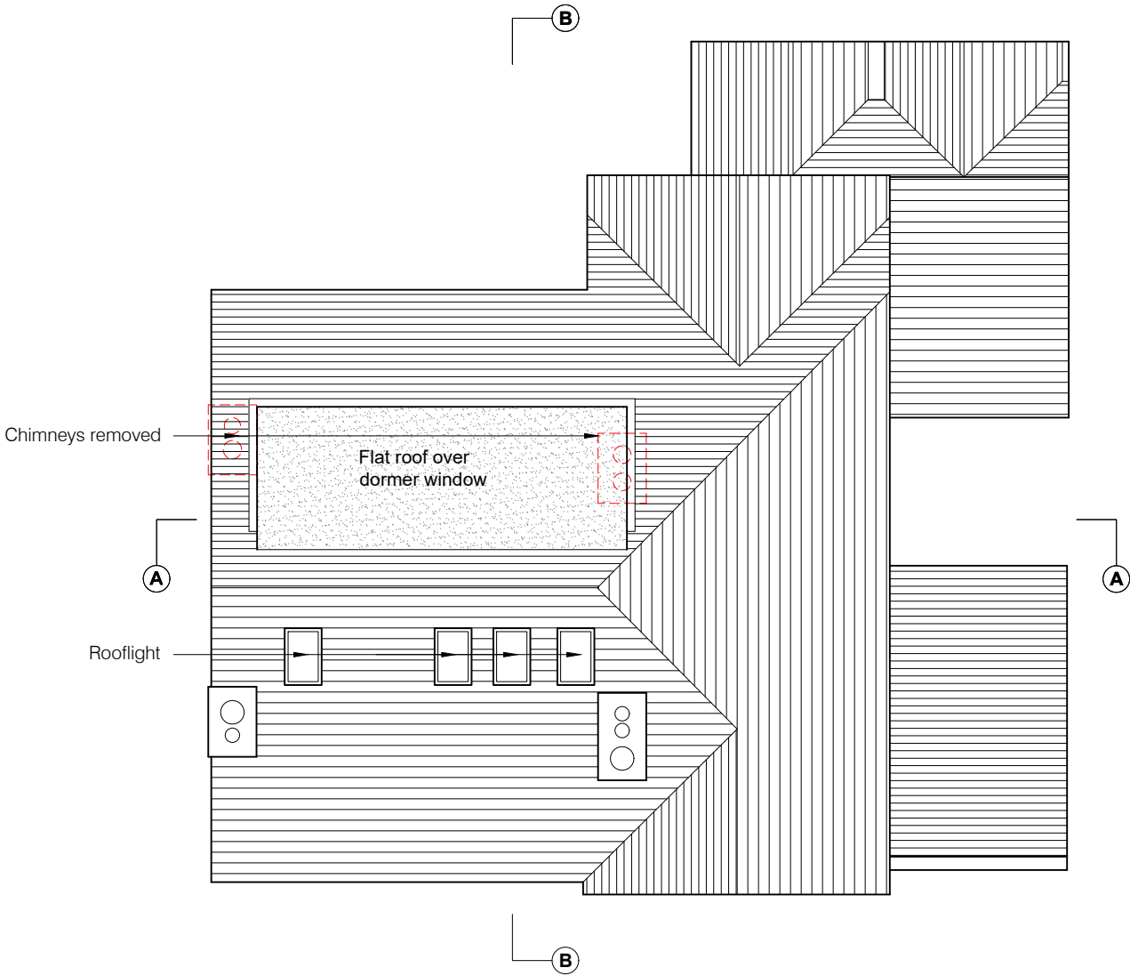
Roof Plan
