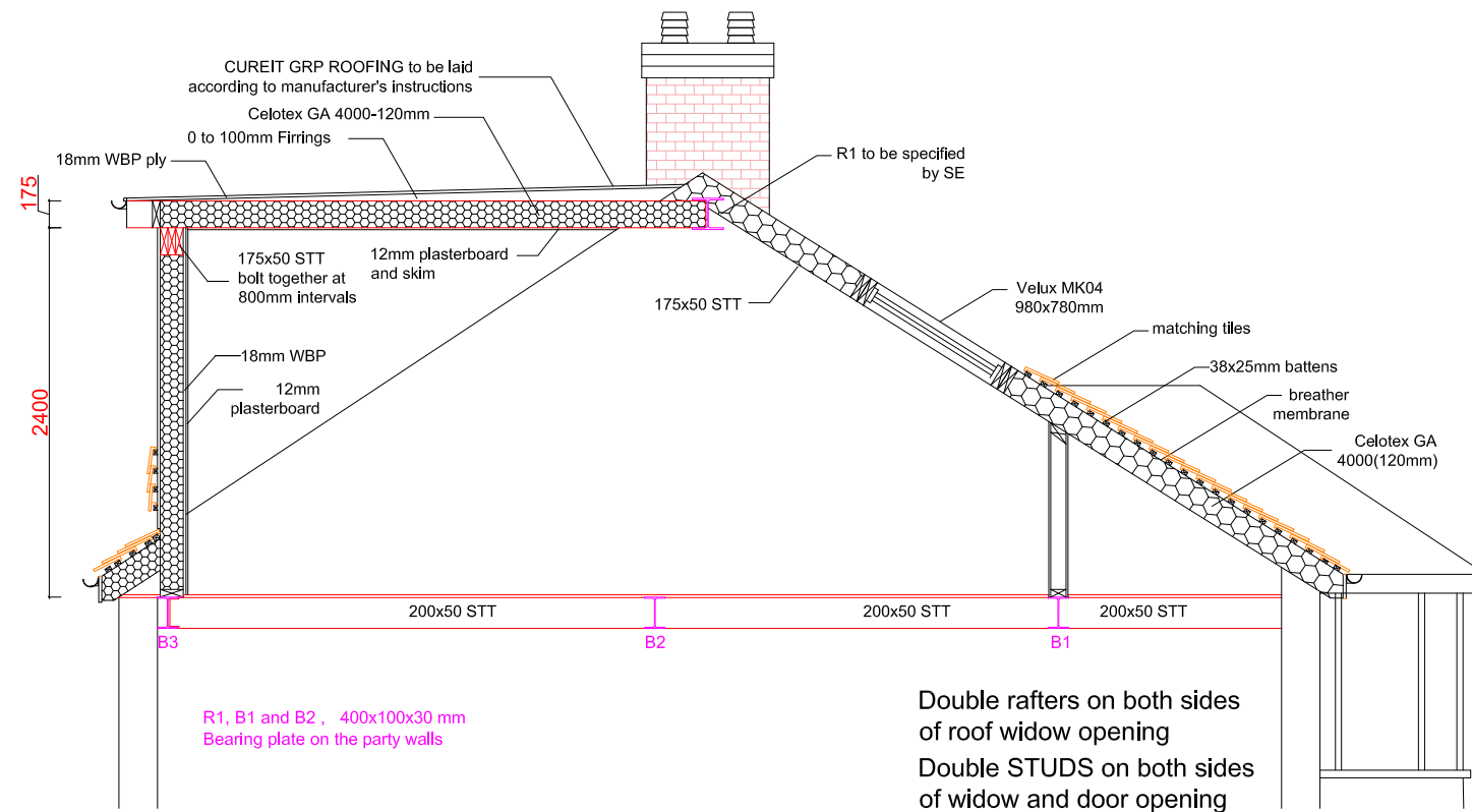
ROOF CONSTRUCTION
