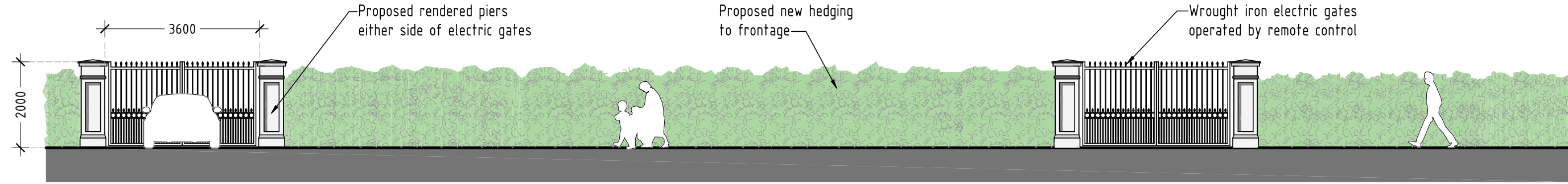
TYPICAL ELEVATION OF GATES & PIERS SCALE 1 : 100
