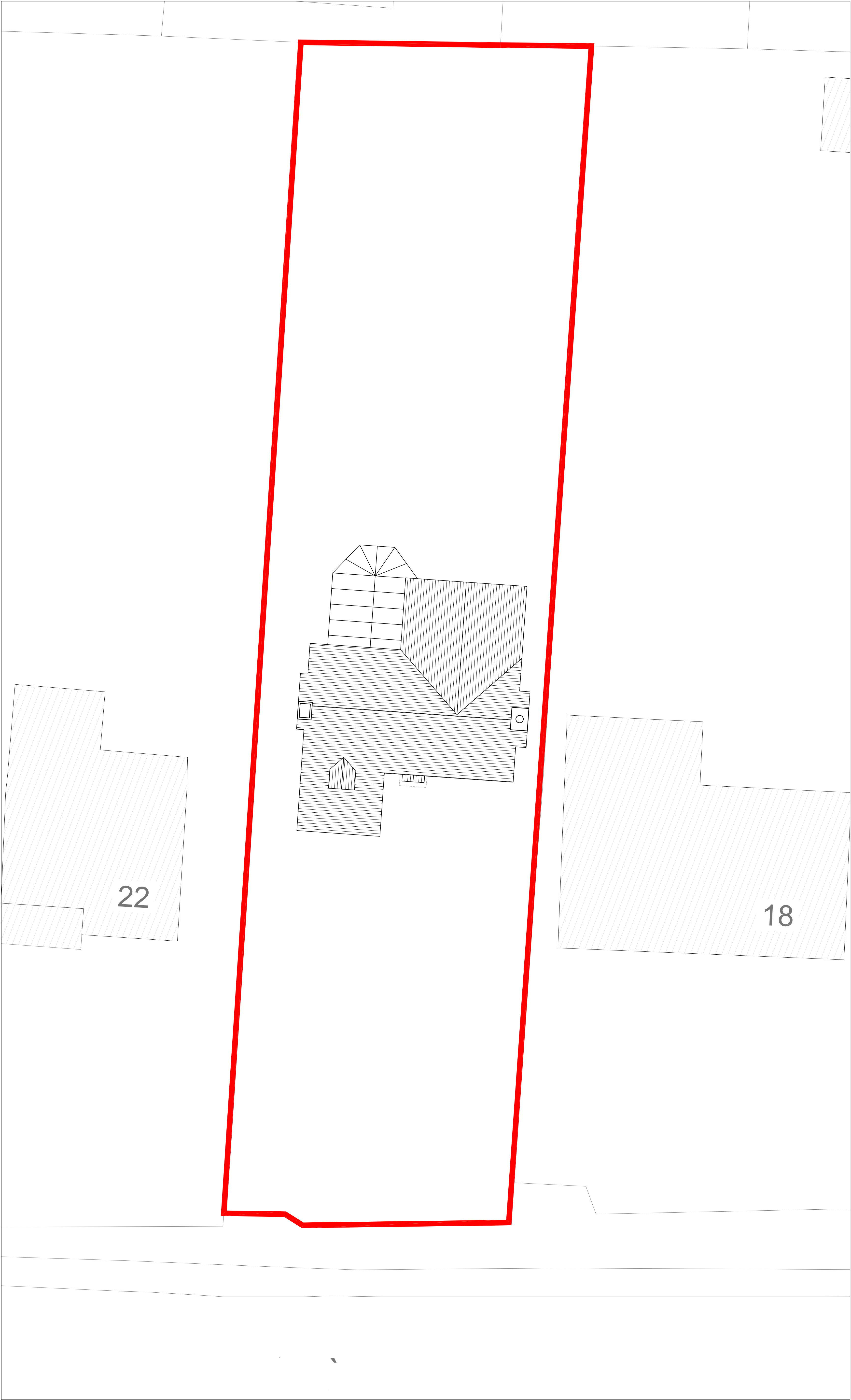
EXISTING BLOCK PLAN SCALE 1:100
