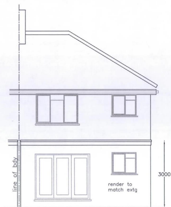
Rear Elevation 1:100
