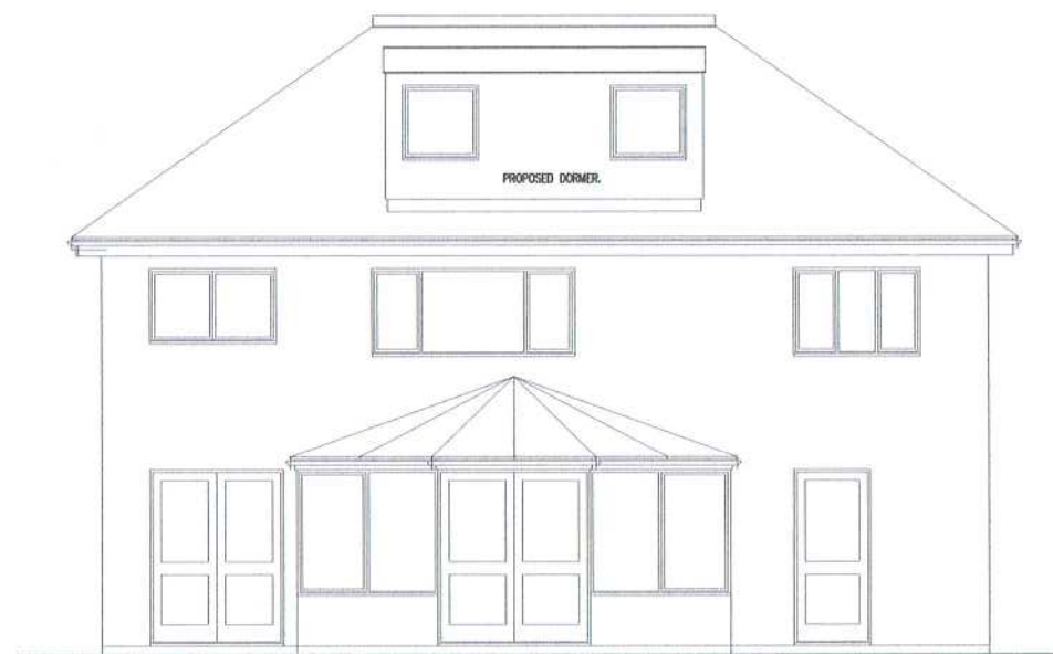
WEST ELEVATION.
