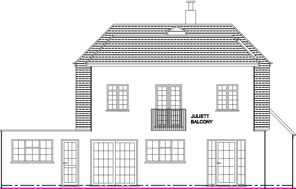
REAR ELEVATION
