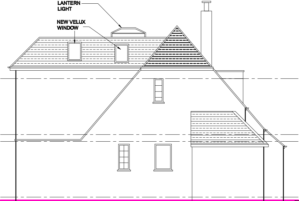
SIDE ELEVATION (FACING NO.24)
