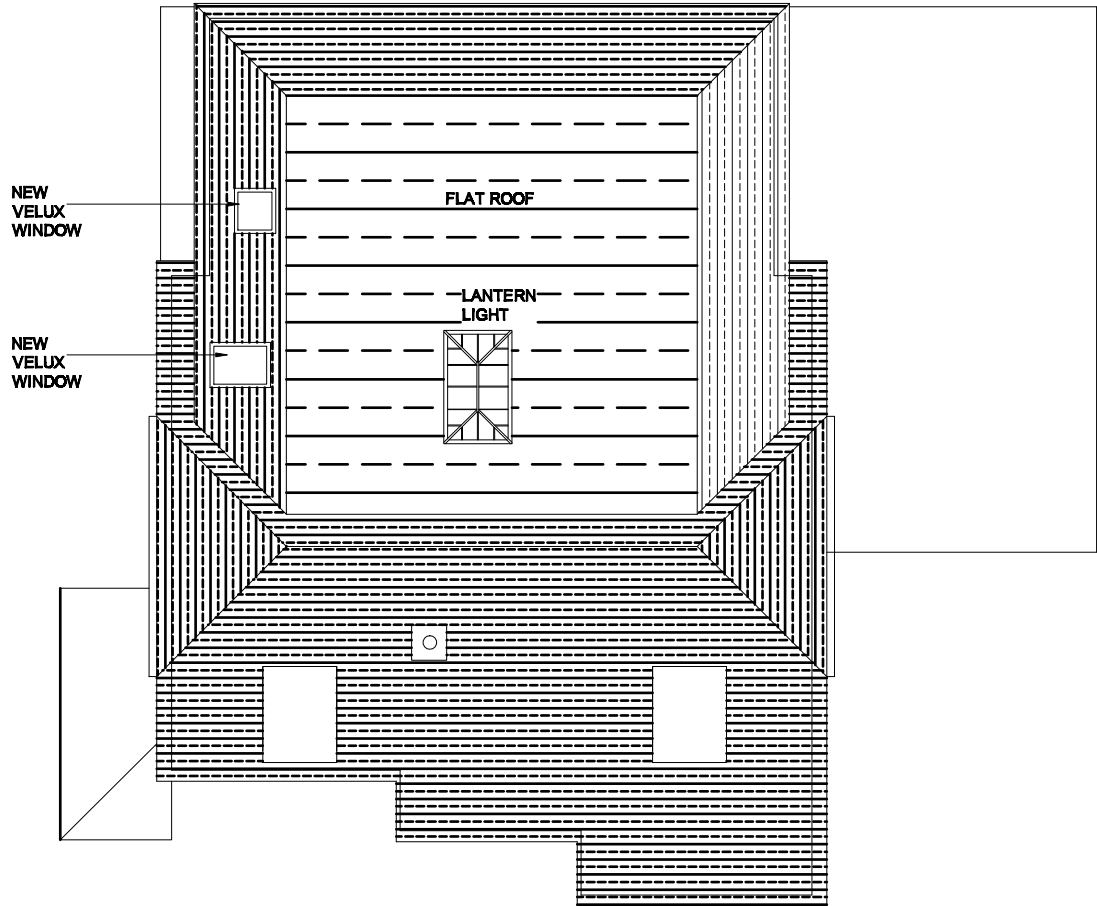
ROOF PLAN
