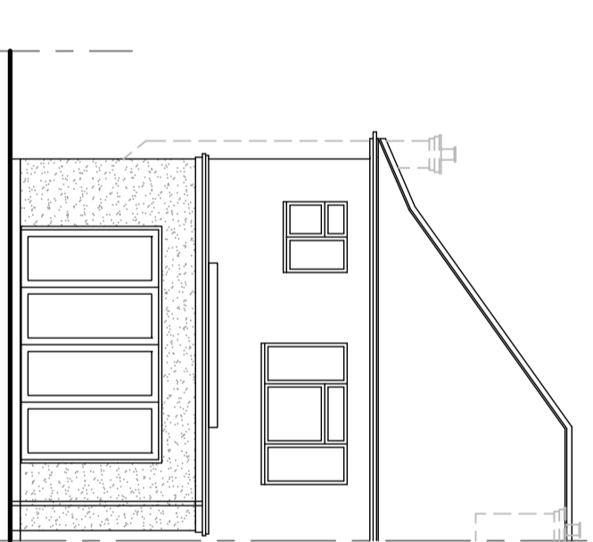
REAR ELEVATION
