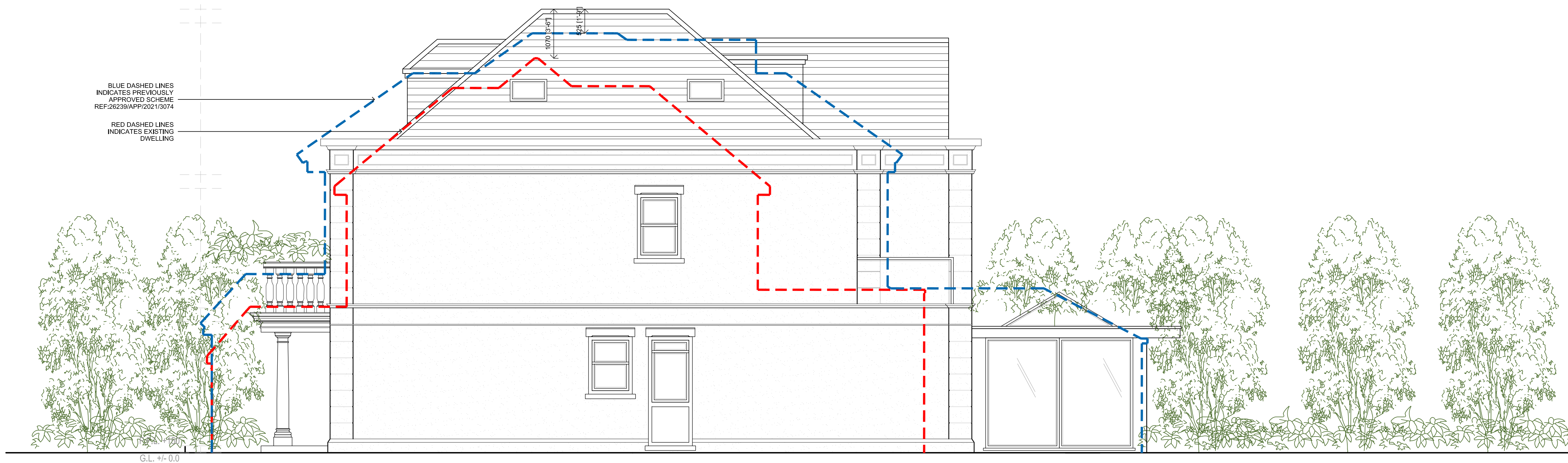
PROPOSED SIDE EAST ELEVATION
