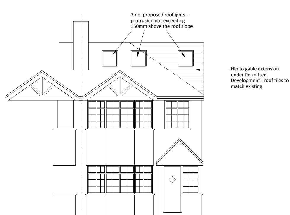
FRONT ELEVATION (WEST) PROPOSED
