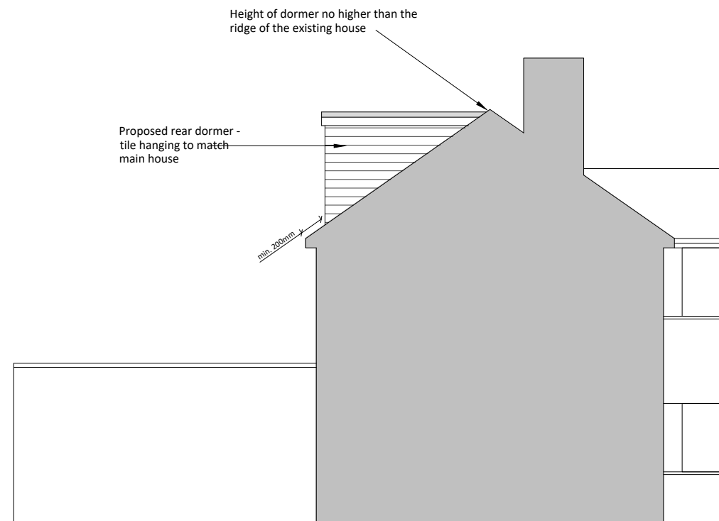
SIDE ELEVATION (SOUTH) PROPOSED
