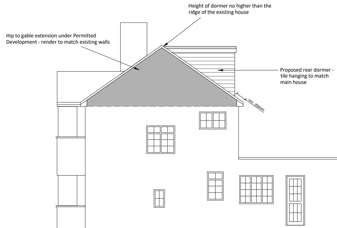
SIDE ELEVATION (SOUTH) PROPOSED
