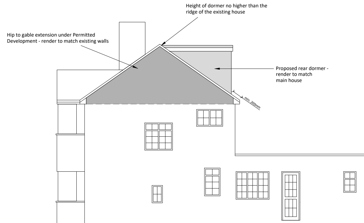
SIDE ELEVATION (SOUTH) PROPOSED
