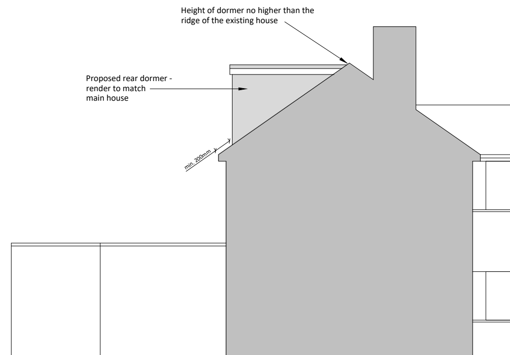
SIDE ELEVATION (NORTH) PROPOSED
