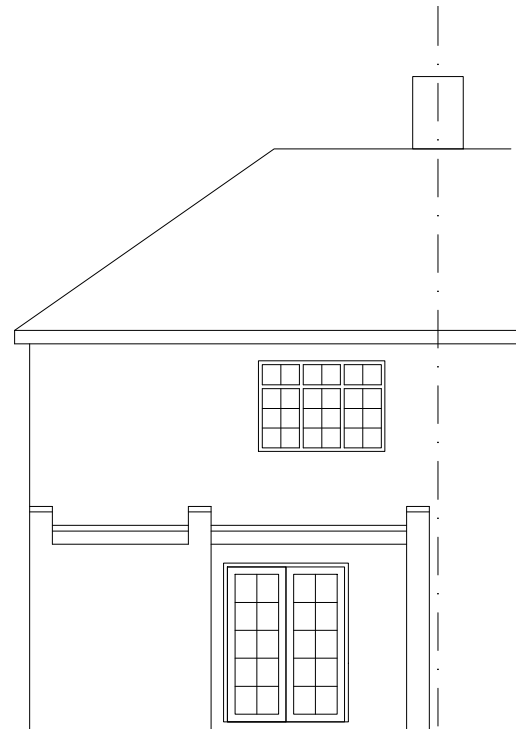
FRONT ELEVATION (WEST)
