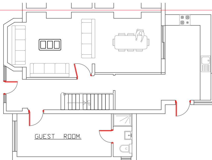
EXISTING GROUND FLOOR
