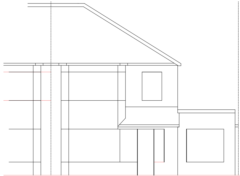
EXISTING FRONT
