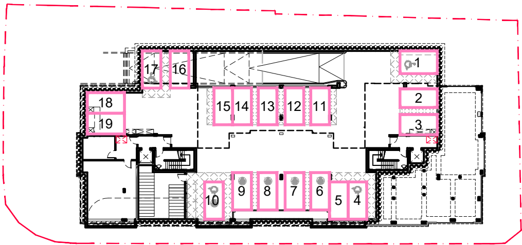
1 BASEMENT PARKING PLAN 902 1:500
