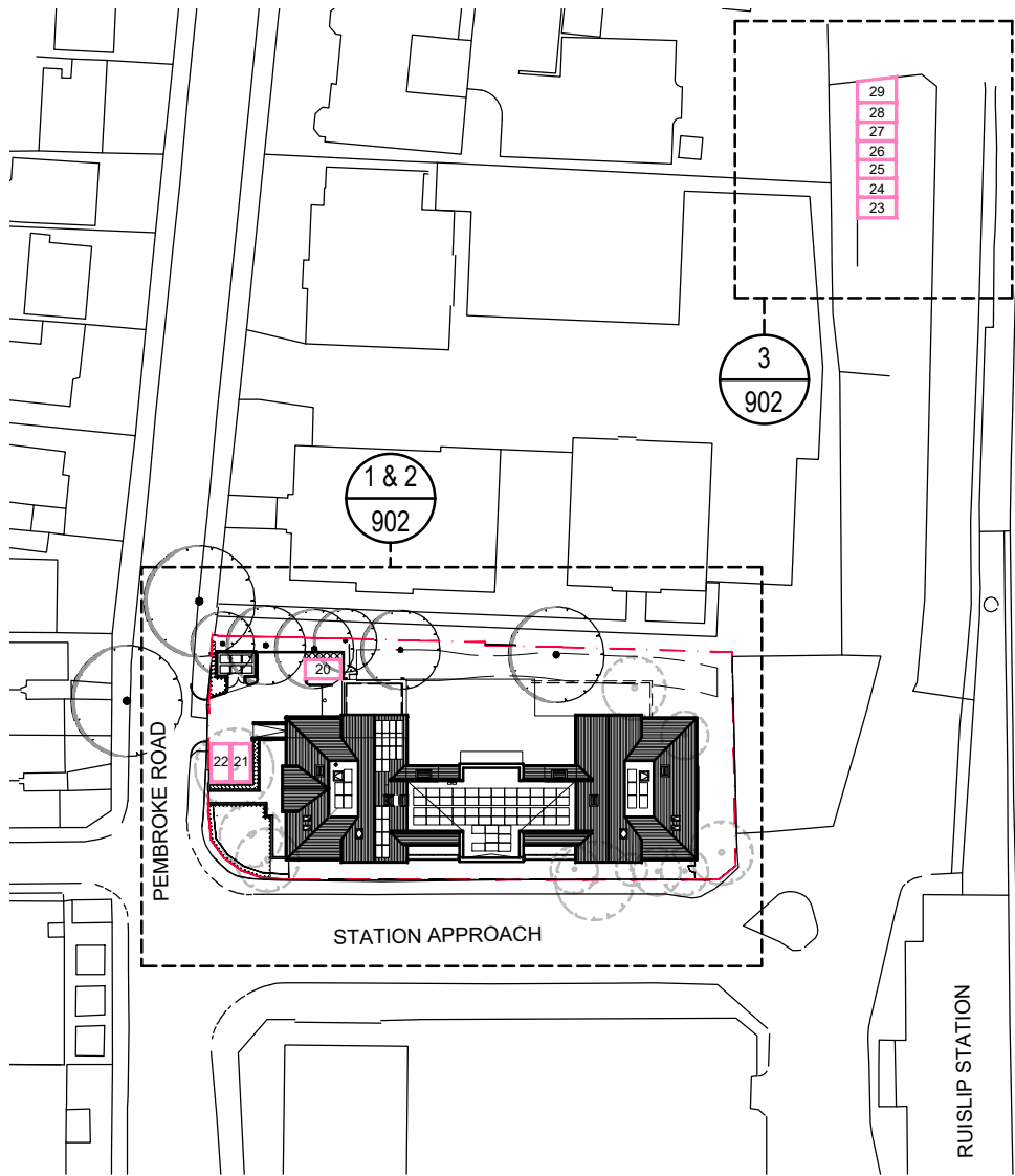
2 KEY PLAN 902 1:1000
