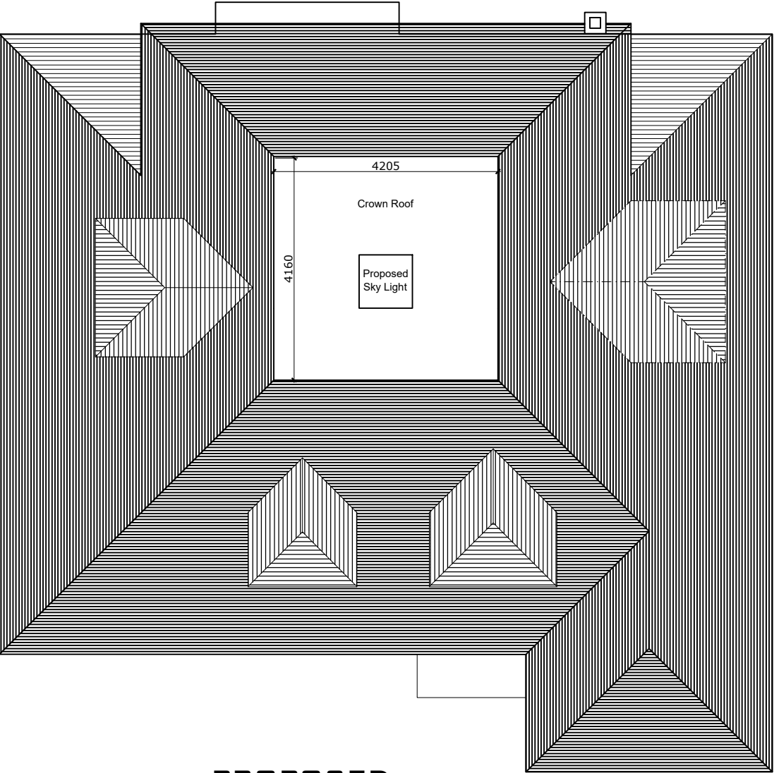
PROPOSED ROOF PLAN S C A L E : 1 : 1 0 0
