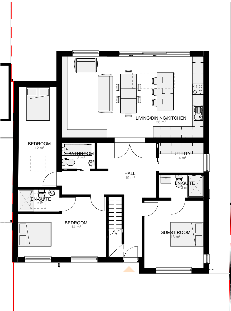
GROUND FLOOR 1 : 100
