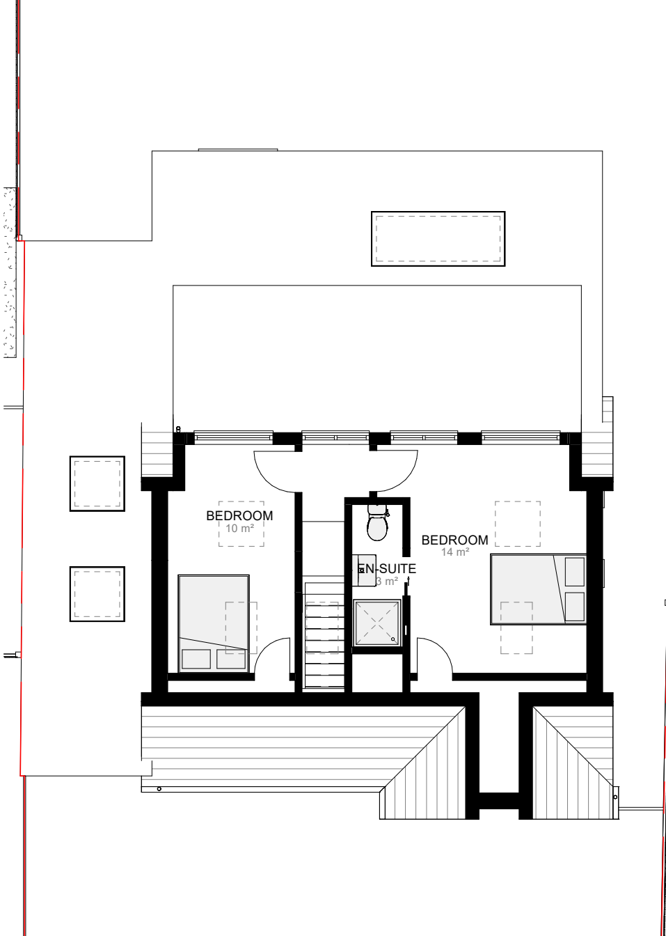
FIRST FLOOR 1 : 100
