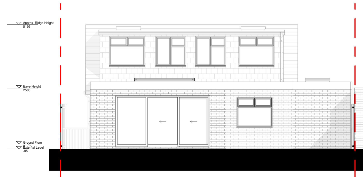
REAR ELEVATION (NORTH-EAST) 1 : 100
