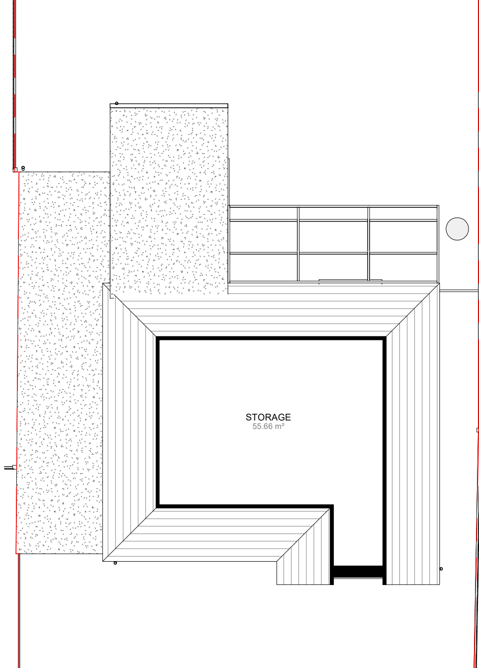
FIRST FLOOR 1 : 100
