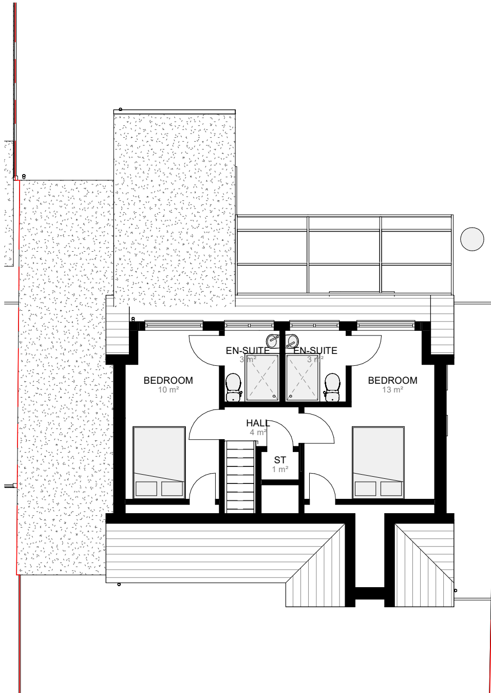
FIRST FLOOR 1 : 100
