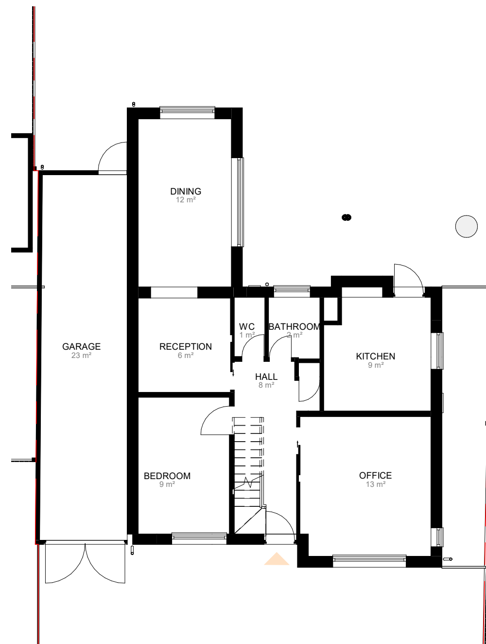
GROUND FLOOR 1 : 100
