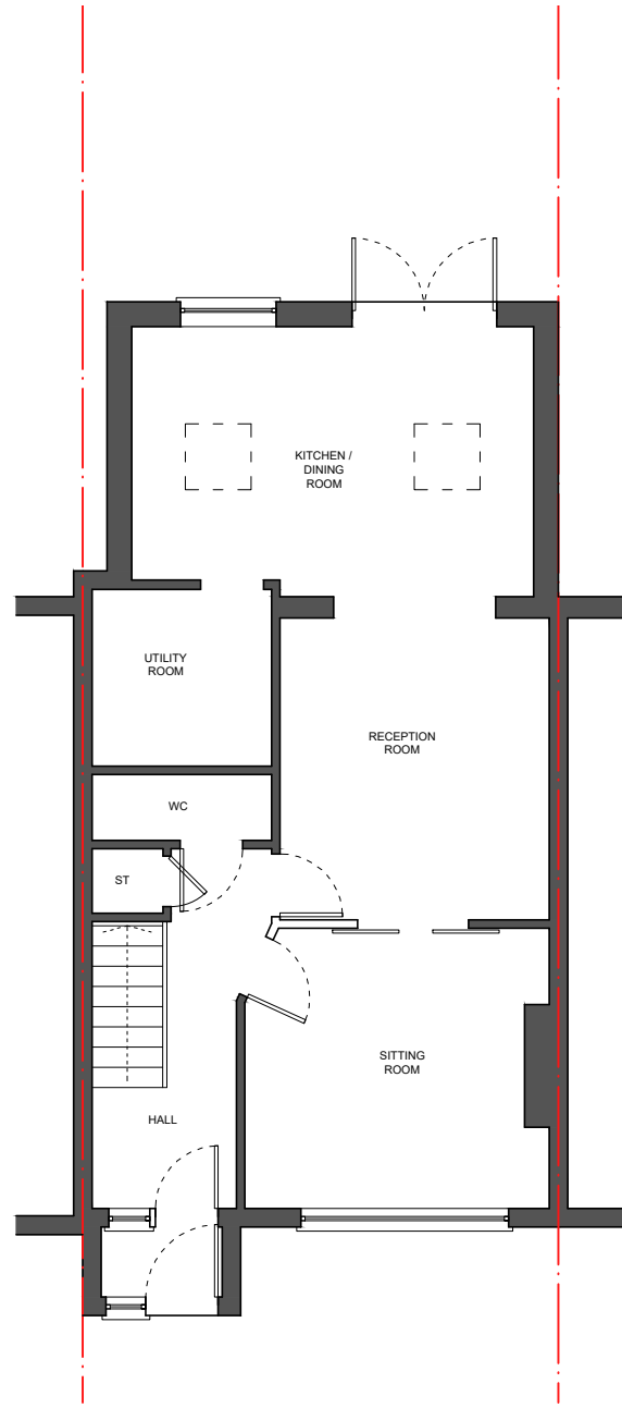
1 EXISTING GROUND FLOOR
