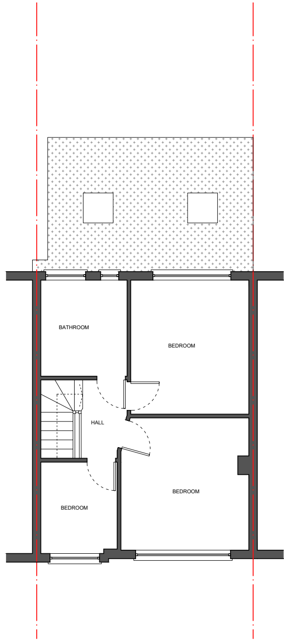
2 EXISTING FIRST FLOOR
