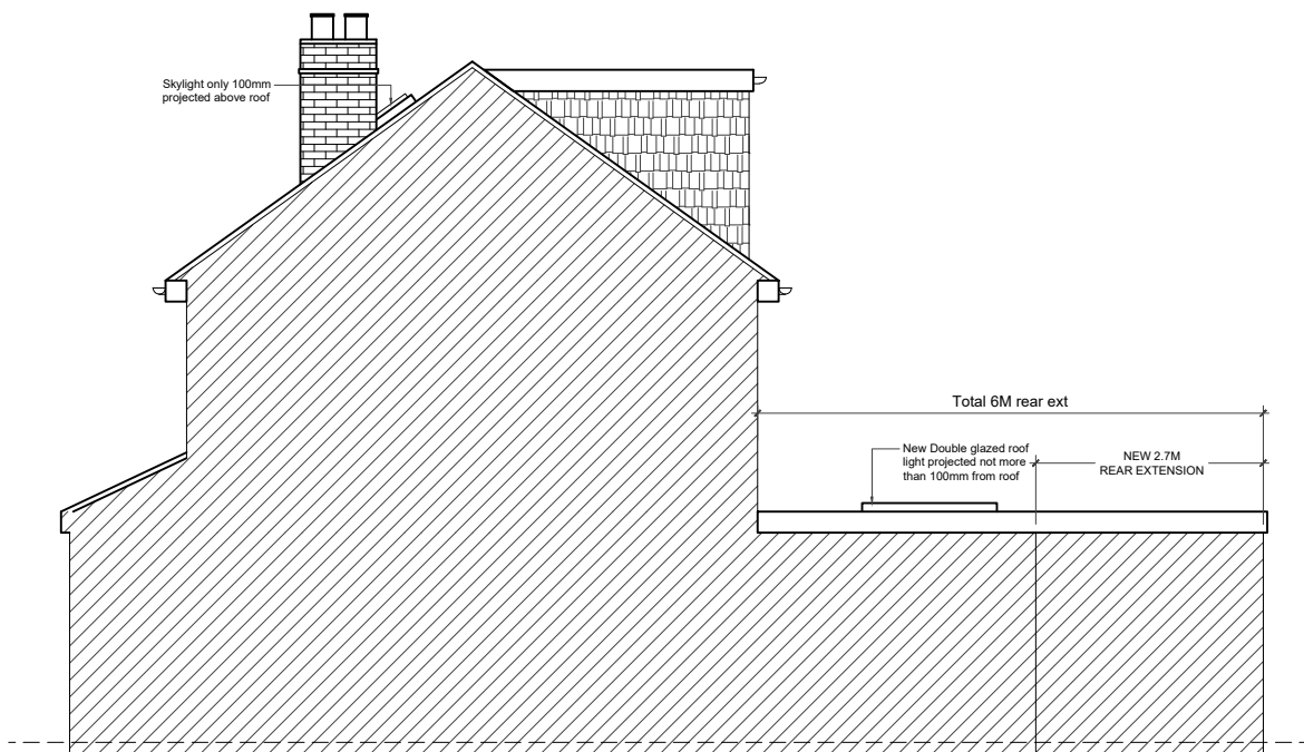
03 - RIGHT SIDE ELEVATION
