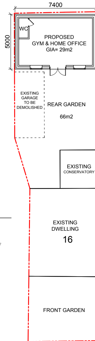
PROPOSED BLOCK PLAN SCALE= 1:200
