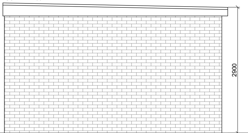
PROPOSED EAST SIDE ELEVATION SCALE= 1:50
