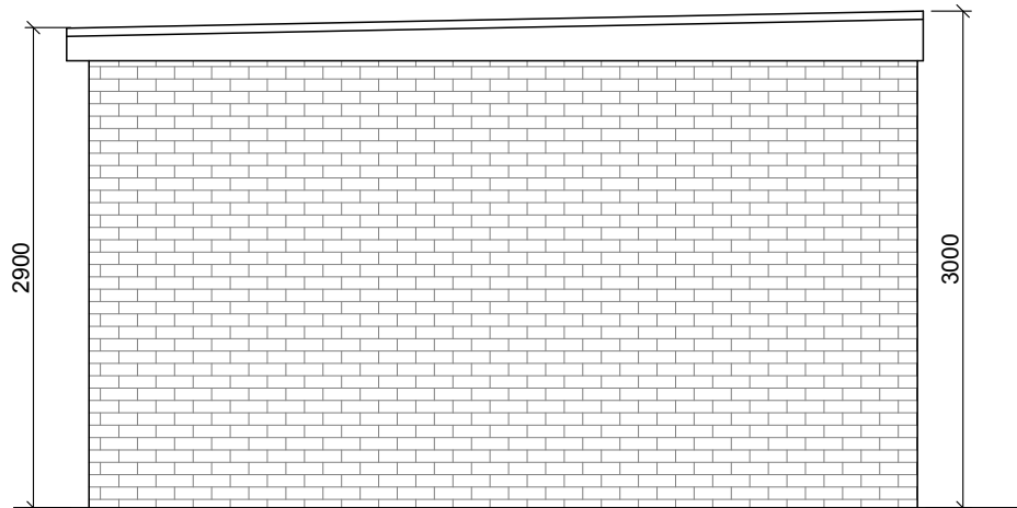
PROPOSED WEST SIDE ELEVATION SCALE= 1:50
